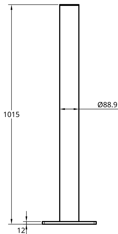
90mm Surface Mount Flat Top Bollard
