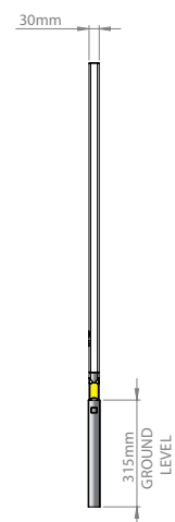
Two Piece Ground Socket
