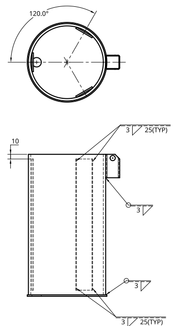
Inground Lockable Socket Assembly
