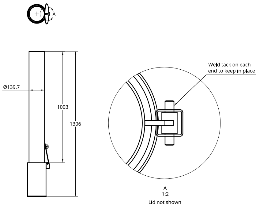
140mm 1000mm Inground Lockable Bollard
