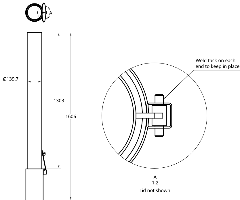
140mm 1300mm Inground Lockable Bollard
